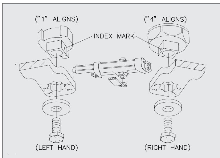
5. Attach the main arm to the closer spindle.
