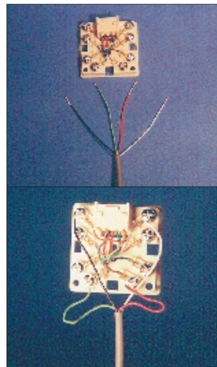
4. A 4-lead splice connects the RJ-31X phone jack to the Telco protector block. The splice wire connects to the phone jack as follows: Splice wire black green red white RJ-31X Jack brown green red gray
