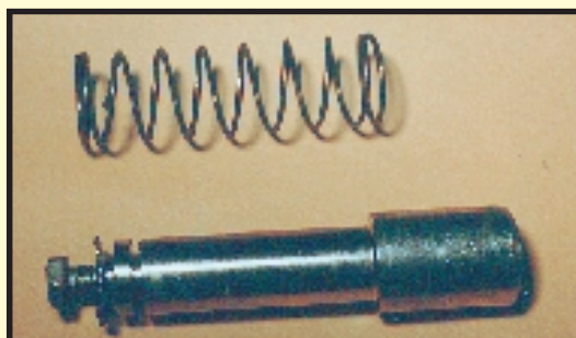
7. The bolt/relocker with high tension spring. Note the slot at the rear of the bolt, next to the mounting bolt. This is the slot for the back cover to attach and move the bolt.
