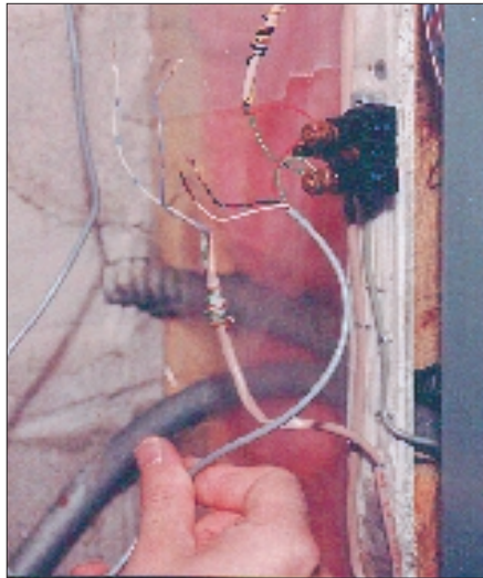
6. The splice wire's green lead and the Telco positive lead are connected to the positive terminal on the Telco block; the splice wire's red lead and the Telco negative lead are connected to the negative terminal.
