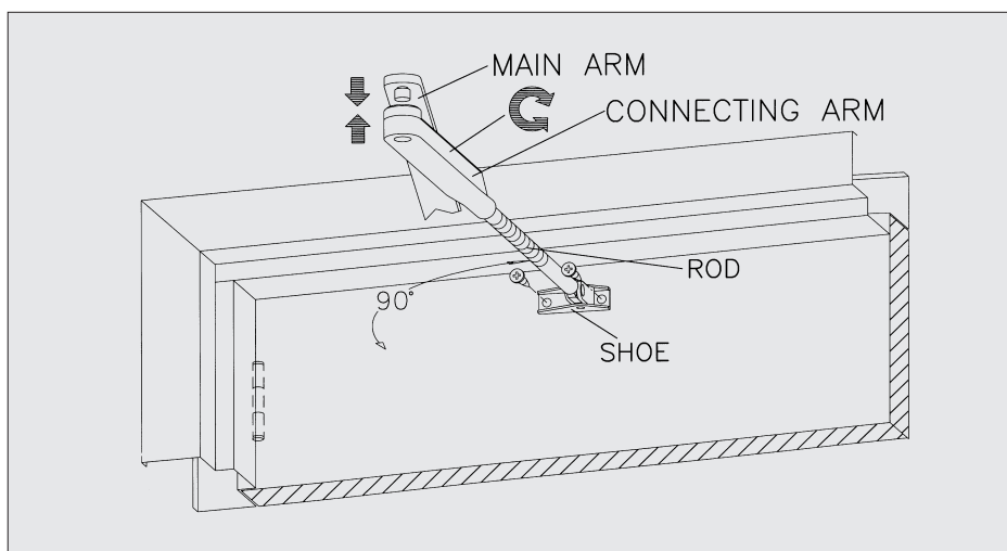
6. Attach the arm shoe to the door, make the necessary adjustments and connect the arm to the main arm.
