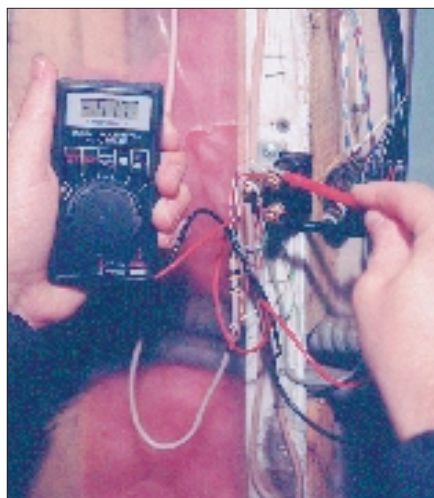
3. The digital voltmeter indicates which Telco terminal is positive and which is negative. This 41.7-volt reading indicates that the bottom terminal (touched by the red lead) is positive. The -41.7 reading indicates that the red lead is touching the negative terminal.
