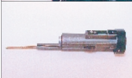
7. Depressing the retainer for lock removal.
