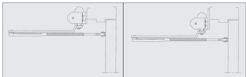
2. When necessary the use of a backplate or drop plate lowers the closer and arm down, providing better clearances when needed.
