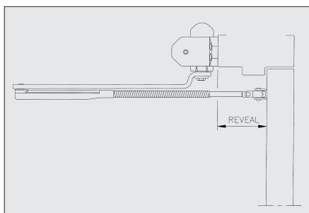
1. The reveal is probably the single biggest differentiation between a standard and top jamb mount. For the top jamb mount, a longer arm is sometimes needed.
