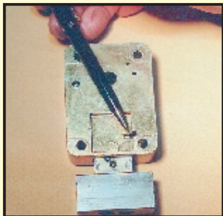
4. The LaGard 3300R combination lock with attached aluminum block. The pen points to the relock trigger.
