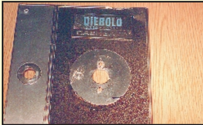
1. Typical Diebold CashGard escutcheon plate with dial mounting holes and hole for opening handle.
