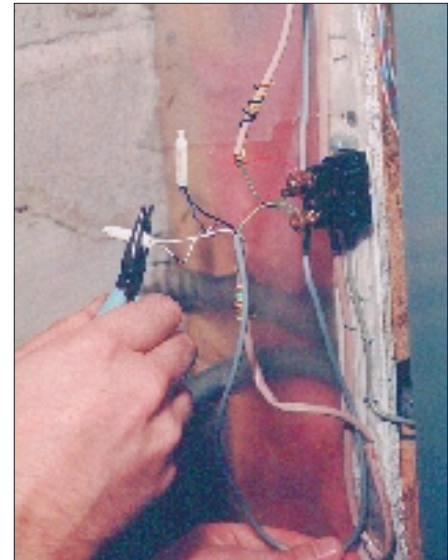
8. The splice wire's white (yellow) lead is connected to the premises phones negative wires.
